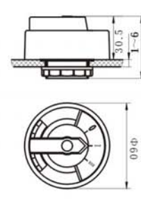
S 开关操作头(大手柄) S Operation head of switch (Large handle)
