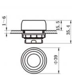
P1 橡胶套按钮操作头 P1 Operation head of rubber sheath button
