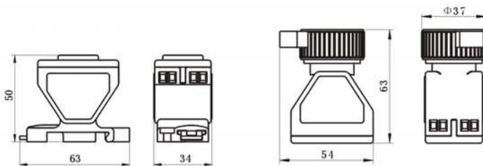
CZ0201 板前型 CZ0201 Board front mounting rail type explosion-proof switch module
