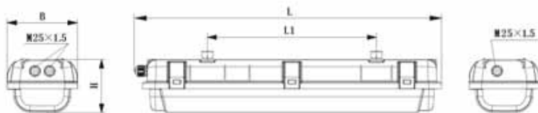
全塑三防荧光灯 Full plastic weather-proof fluorescent light fittings
