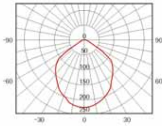
M087D-N70W 高压钠灯 High pressure sodium vapor lamp
