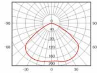
M087D-N250W 高压钠灯 High pressure sodium vapor lamp
