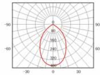
M087D-QL135W 电磁感应节能灯 Electromagnetic induction energy-saving lamp
