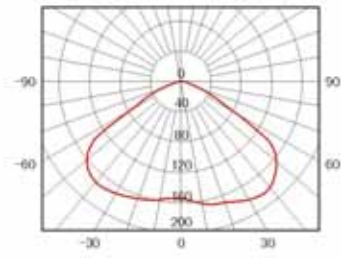
M087D-J400W 金属卤化物灯 Metal halide lamp
