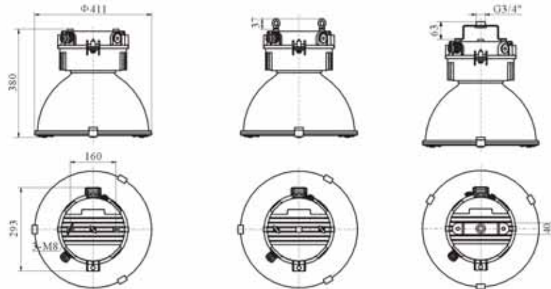
M087D/1 三防高顶灯 M087D/1 Weather-proof high dome light fittings
