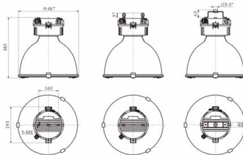
M087D/2 三防高顶灯 M087D/2 Weather-proof high dome light fittings
