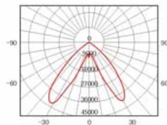
M087D-J1000W 金属卤化物灯 Metal halide lamp MW—中宽配光 MW-Medium wide distribution
