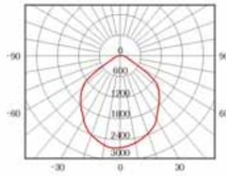
M087D-N100W 高压钠灯 High pressure sodium vapor lamp
