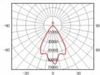
M087D-J1000W 金属卤化物灯 Metal halide lamp MB—中配光 MB-Medium light distribution
