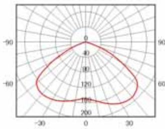
M087D-N400W 高压钠灯 High pressure sodium vapor lamp
