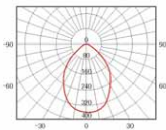
M087D-QL165W 电磁感应节能灯 Electromagnetic induction energy-saving lamp
