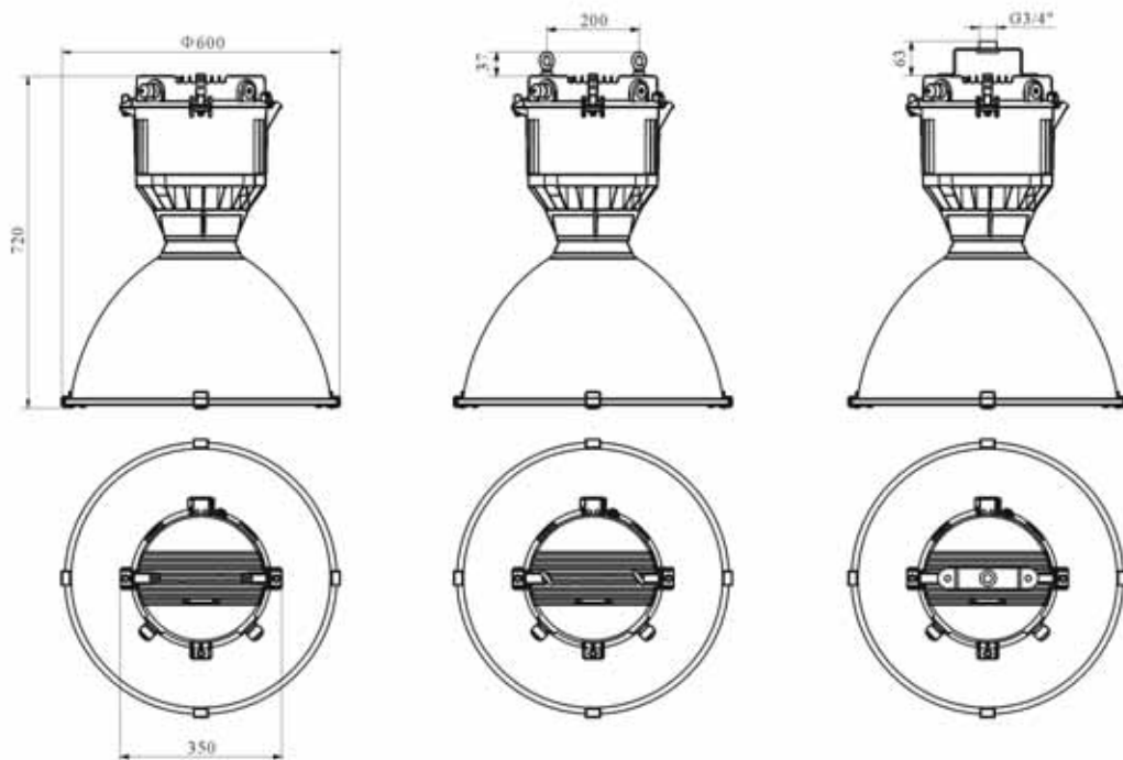
M087D/3 三防高顶灯 M087D/3 Weather-proof high dome light fittings
