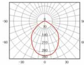
M087D-QL85W 电磁感应节能灯 Electromagnetic induction energy-saving lamp
