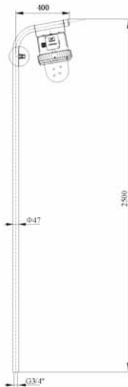
护栏式安装 Fence type
