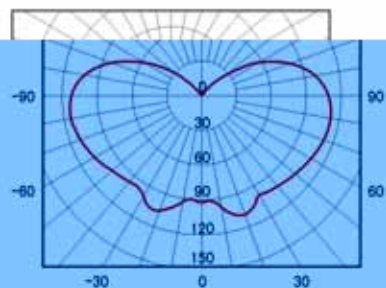
CZ0872-QL135W 电磁感应节能灯 Electromagnetic induction energy-saving lamp
