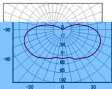
CZ0871-QL50W 电磁感应节能灯 Electromagnetic induction energy-saving lamp
